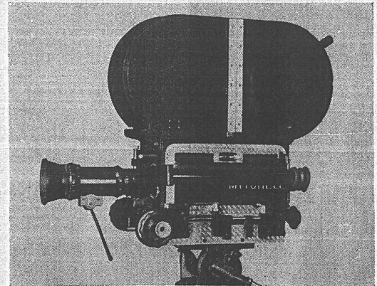
PAN-CINOR Zoom-type lens mounted on Mitchell BNC camera. Finder tube extends to rear.
